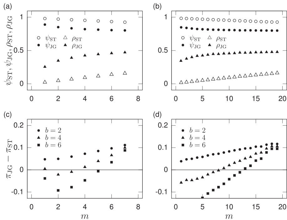
Figure 7 Equilibria for a population of DISC players under heterogeneous assignment rules. (a), (b) Cooperativeness ( \psi_{ST} and \psi_{JG} ) and ingroup bias ( \rho_{ST} and \rho_{JG} ) for groups employing ST and JG. (c), (d) Payoff difference between a player in a ST group and that in a JG group ( \pi_{JG} - \pi_{ST} ). We set \theta = 0.6 and c = 1 . We also set M = 8 in (a) and (c) , M = 20 in (b) and (d) , and vary the number of JG groups (i.e., m ) and b .
